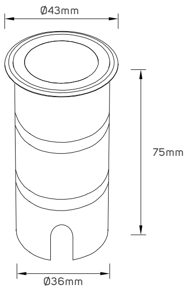
LI615356 (Cutting size \varnothing 36 )
