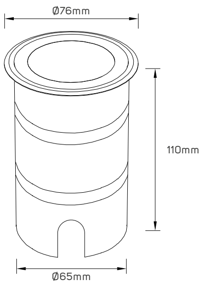
LI615359-LI615360-LI615361-LI615362-LI615363 (Cutting size \varnothing 65 )
