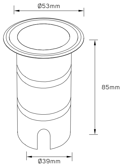
LI615357 (Cutting size \varnothing 39 )
