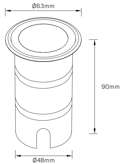
LI615358 (Cutting size \varnothing 48 )
